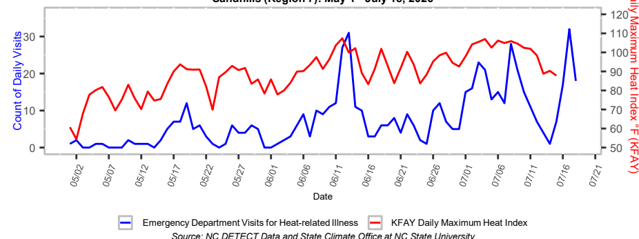
Figure 3. Emergency Department Visits for Heat-related Illness and Daily Maximum Heat Index Sandhills (Region 7): May 1 - July 18, 2026
