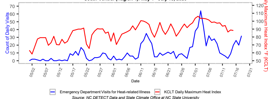
Figure 3. Emergency Department Visits for Heat-related Illness and Daily Maximum Heat Index South Central (Region 4): May 1 - July 18, 2026
