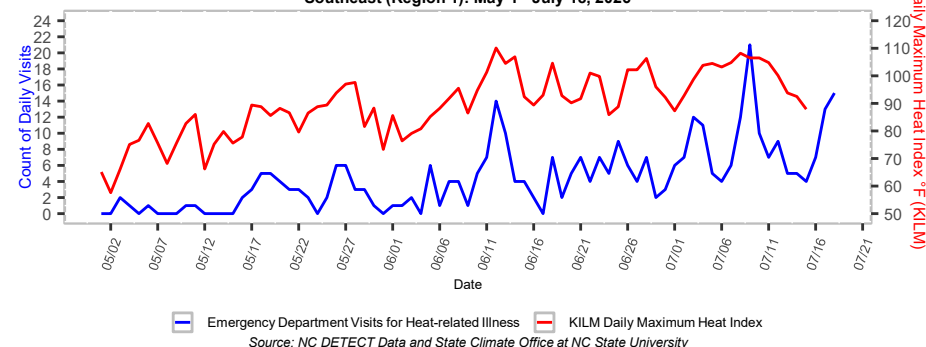
Figure 3. Emergency Department Visits for Heat-related Illness and Daily Maximum Heat Index Southeast (Region 1): May 1 - July 18, 2026
