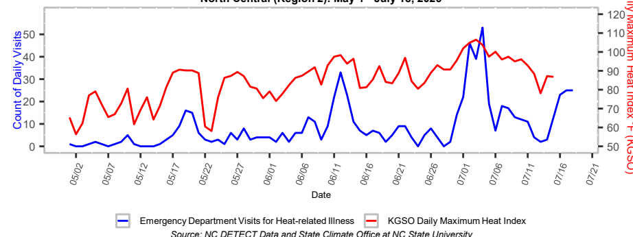
Figure 3. Emergency Department Visits for Heat-related Illness and Daily Maximum Heat Index North Central (Region 2): May 1 - July 18, 2026
