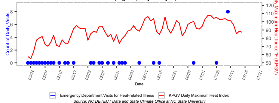
Figure 3. Emergency Department Visits for Heat-related Illness and Daily Maximum Heat Index Northeast (Region 3): May 1 - July 18, 2026
