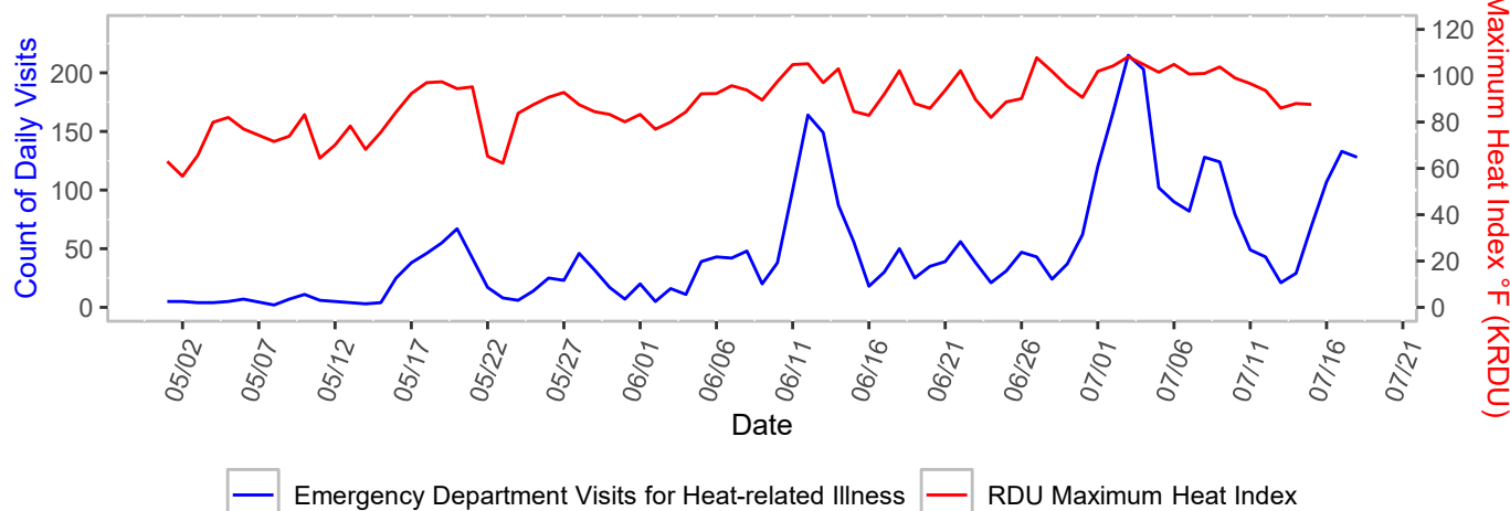
Figure 3. Emergency Department Visits for Heat-related Illness and Maximum Heat Index North Carolina Statewide: May 1 - July 18, 2026
