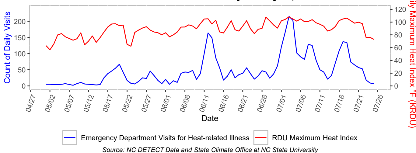
Figure 3. Emergency Department Visits for Heat-related Illness and Maximum Heat Index North Carolina Statewide: May 1 - July 25, 2026
