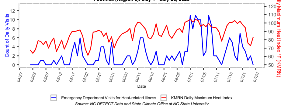
Figure 3. Emergency Department Visits for Heat-related Illness and Daily Maximum Heat Index Foothills (Region 6): May 1 - July 25, 2026
