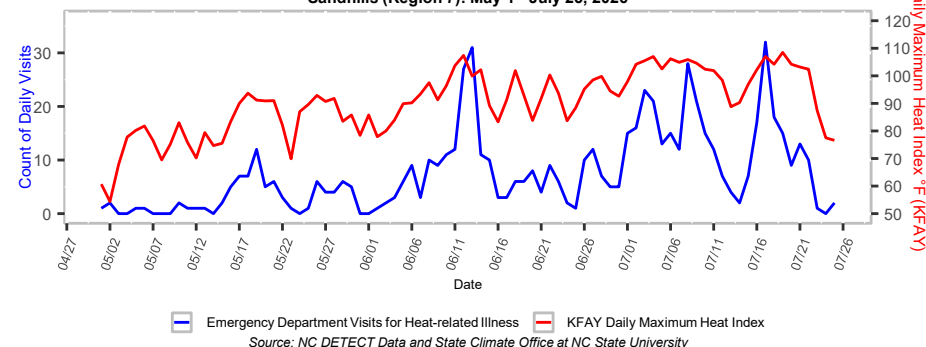
Figure 3. Emergency Department Visits for Heat-related Illness and Daily Maximum Heat Index Sandhills (Region 7): May 1 - July 25, 2026
