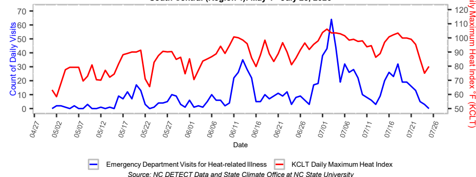
Figure 3. Emergency Department Visits for Heat-related Illness and Daily Maximum Heat Index South Central (Region 4): May 1 - July 25, 2026
