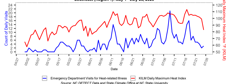
Figure 3. Emergency Department Visits for Heat-related Illness and Daily Maximum Heat Index Southeast (Region 1): May 1 - July 25, 2026
